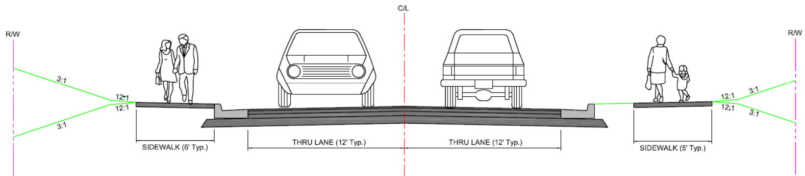
Typical Cross Section Options
